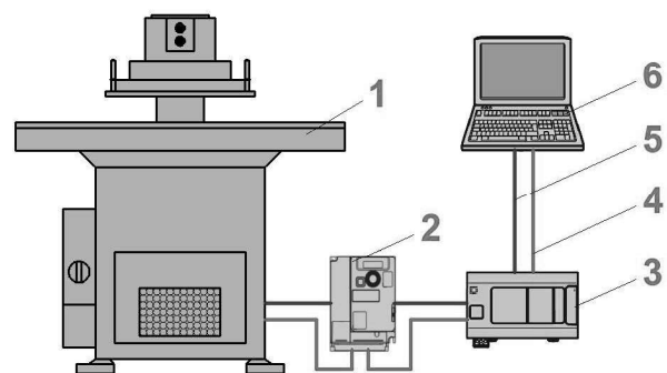
Figure 1 Experimental scheme for parameters investigation of press equipment: 1 – cutting press Atom SE20C; 2 – frequency converter Altivar 320 ATV320U15N4C; 3 – measuring unit WB-1; 4 - line of direct connection; 5 - line of feedback connection; 6 - PC
